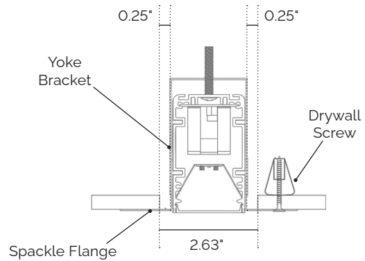
SFY (Yoke Mount)
