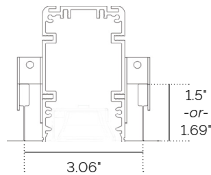
15/16" T-Bar Flush
