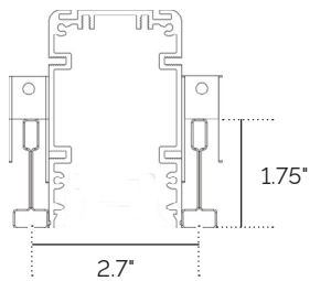
9/16" T-Bar Bolt Slotted
