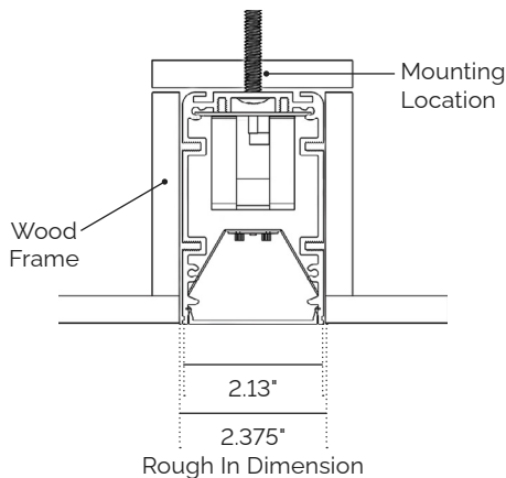
TR (Screw / Rod Mount)
