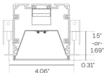
15/16" T-Bar Tegular
