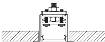
CB Screw/Rod Mount
