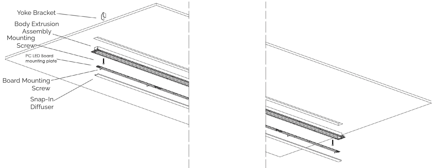
Drywall Ceiling Mounting Shown with Spackle Flange
