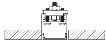
TR 2 Trimless
