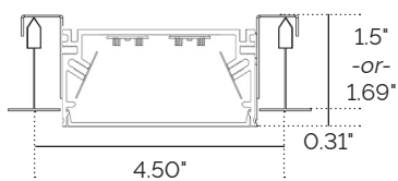
15/16" T-Bar Tegular
