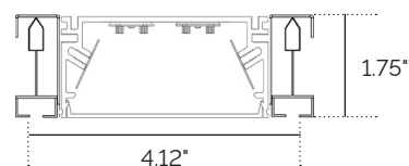
9/16" T-Bar Bolt Slotted
