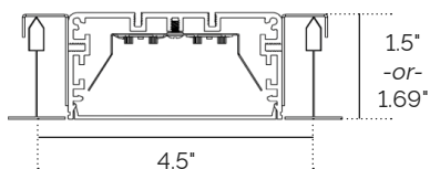
15/16" T-Bar Flush
