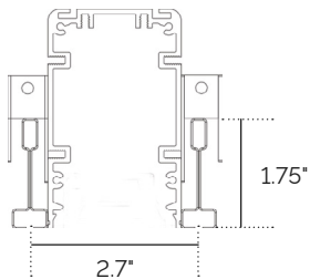
9/16" T-Bar Bolt Slotted
