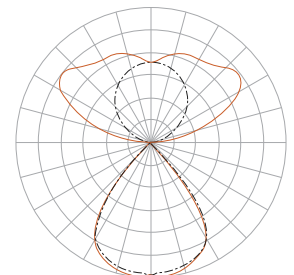
Indirect: Batwing (BW) Direct: 80° Reflector
