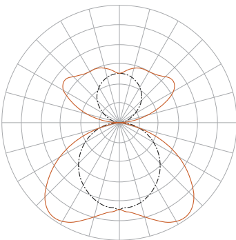
Indirect: Batwing (BW) Direct: Wide Diffuse (WD)
