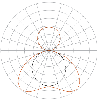
Indirect: Clear (CL) Direct: Wide Diffuse (WD)
