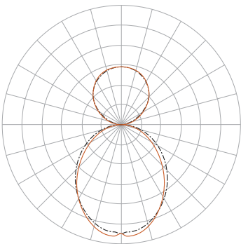
Indirect: Clear (CL) Direct: SatinIce Diffuse (SD)
