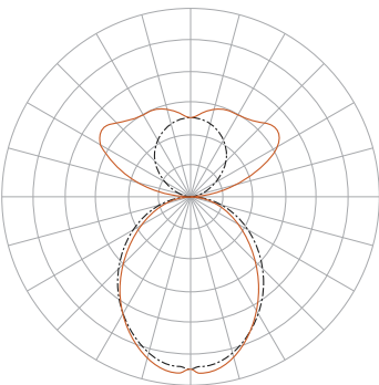
Indirect: Batwing (BW) Direct: SatinIce Diffuse (SD)
