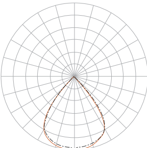
Direct: 80° Reflector
