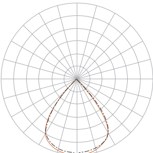
Direct: 80° Reflector
