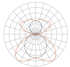
Indirect: Batwing (BW) Direct: Wide Diffuse (WD)
