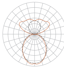
Indirect: Batwing (BW) Direct: SatinIce Diffuse (SD)
