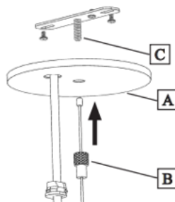
Power feed side. Secure canopy (A) with threaded coupler (B) on threaded stud (C)
