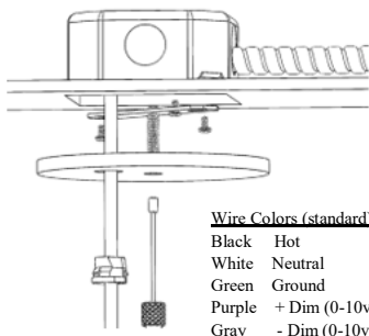
Power feed side. Secure canopy (A) with threaded coupler (B) on threaded stud (C)
