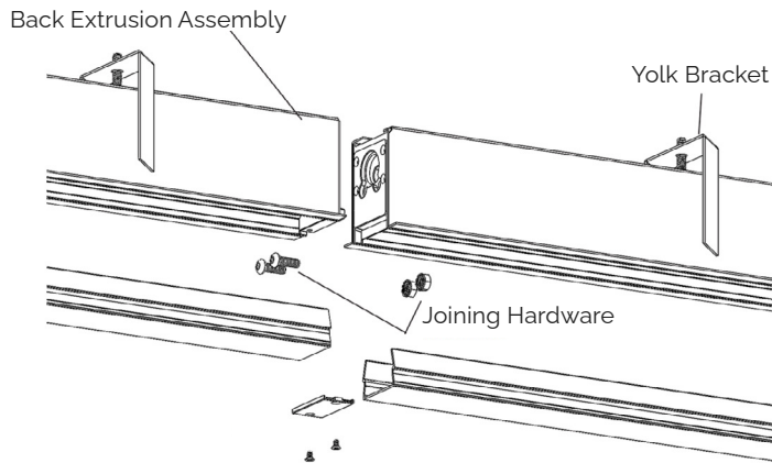
Joiner Detail
