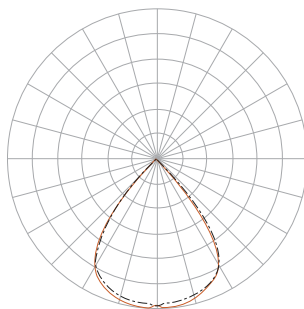
Direct: 80° Reflector
