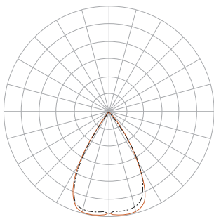
Direct: 50° Reflector
