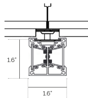
TB4 15/16" Tegular
