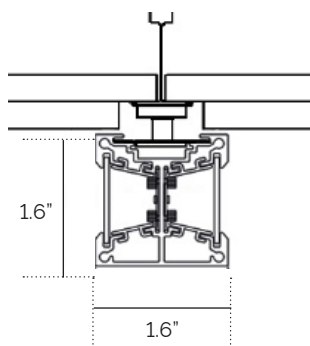
TB3 9/16" Tegular
