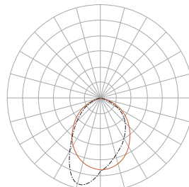
Direct: Wall Wash (WW)
