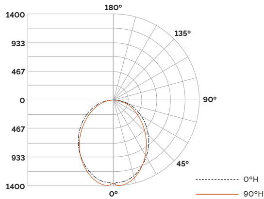
SLIMD-4-750-SD-35K (80+ CRI)
