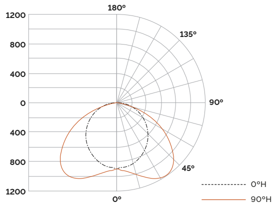
SLIMD-4-750-WD-35K (80+ CRI)
