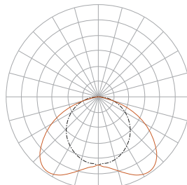
Direct: Wide Diffuse (WD)
