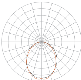
Direct: Satinice Diffuse (SD)
