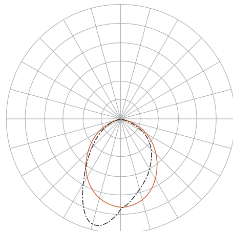
Direct: Wall Wash (WW)
