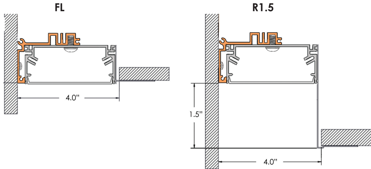
Mounting Length end Detail
