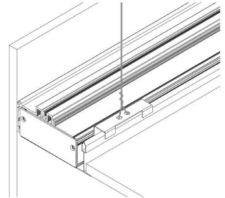
Universal Hole Pattern Side clip has a universal hole pattern to match many t-grid styles.
