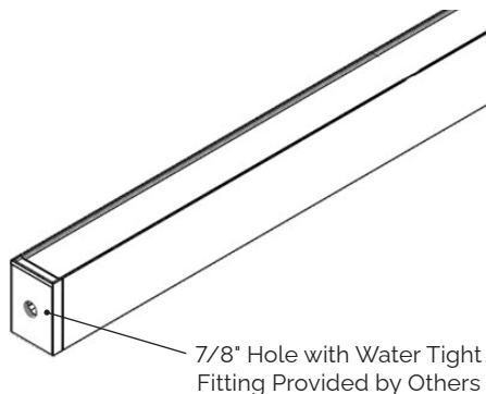
SM(E) (End-Fed Power Stem Mount)
