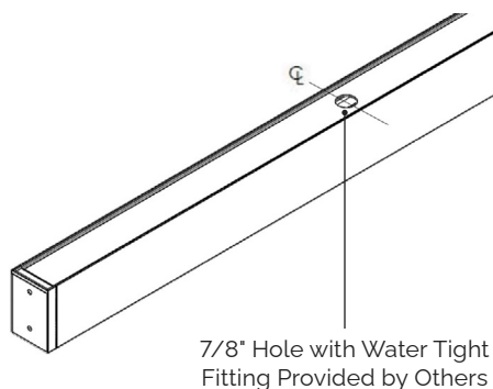
SM(T) (Top-Fed Power Stem Mount)
