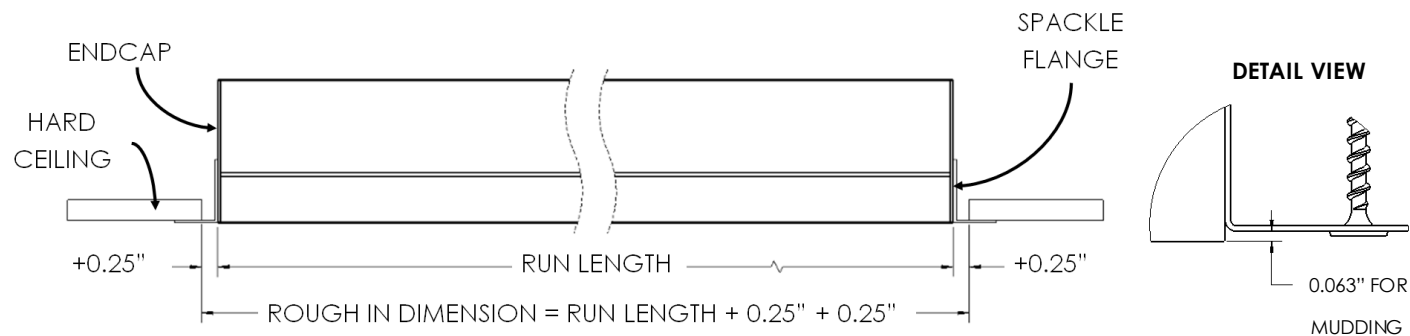
Mounting Length end Detail
